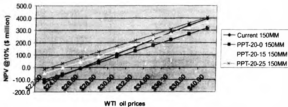
Chart 5.14. NPV @10% for a 150 million barrel field - low well productivity, high costs
