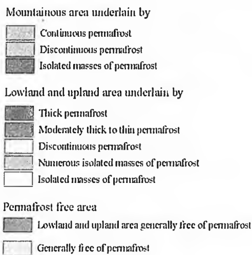
Fig. 4. Permafrost regions of Alaska (Ferrians, O. J., 1965, Permafrost map of Alaska, digital data pulled from the Alaska Geospatial Data Clearinghouse, http://agdc.usgs.gov )
