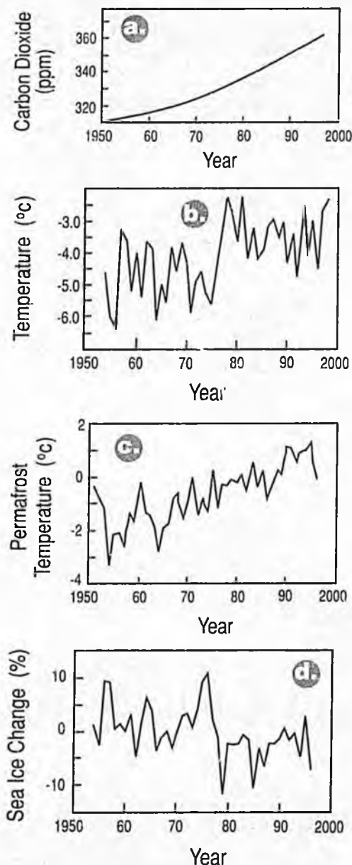
Fig. 1. Climate and climate-related trends in Alaska. a) CO 2 at Barrow, Alaska (smoothed), b) annual mean temperature composite from Anchorage, Fairbanks, Nome and Barrow, c) permafrost temperatures at Fairbanks, d) change in sea ice extent (%) in the Bering Sea.
