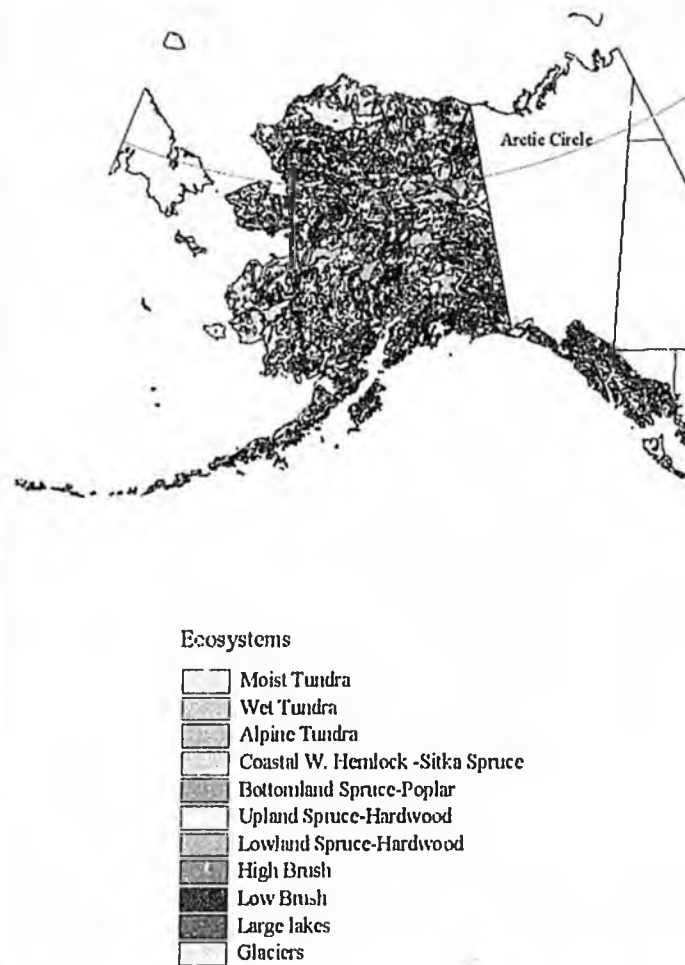
Fig. 3. Ecosystems of Alaska (Joint Federal-State Land Use Planning Commission for Alaska, 1973)
