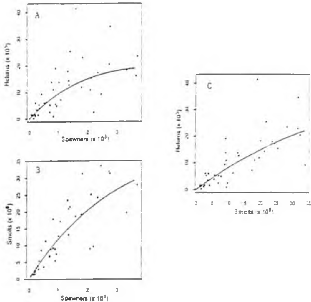
Figure 11-2 Ricker stock-recruitment data and functions for Chilko Lake sockeye salmon from Fraser River. A, adult spawners and adult returns; B, adult spawners and juvenile downstream migrants (age 1 - smolts); and C, migrants and adult returns.
