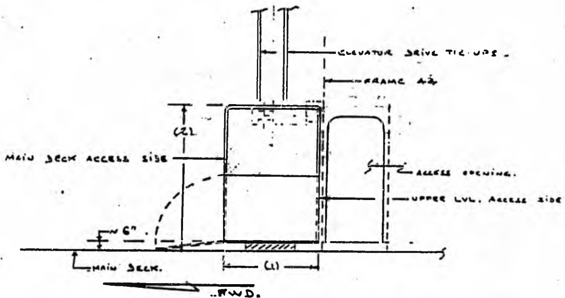
PROFILE ELEVATION, FROM CENTERLINE LOOKING TO STARBOARD.
