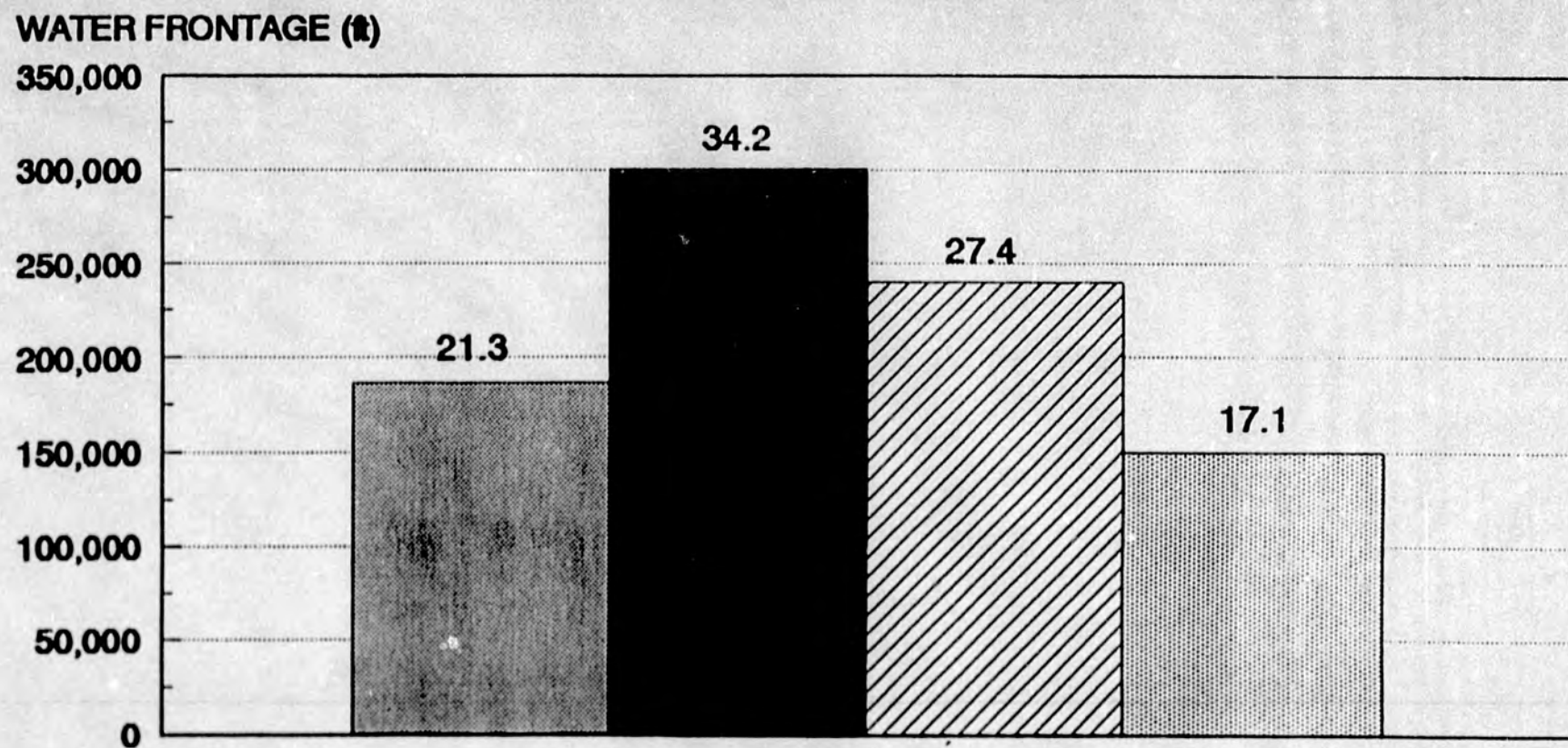
FIG. 23 KENAI RIVER NEARSHORE SUBSTRATES ALL REACHES COMBINED
