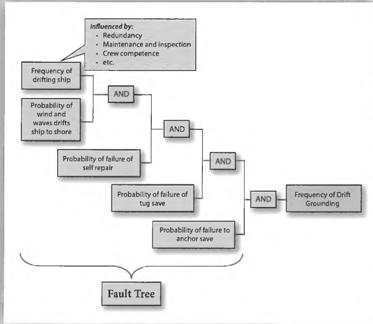
Figure 11. Fault tree for drift grounding accidents.
