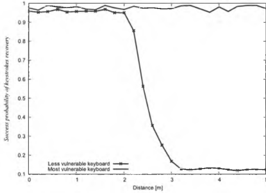
Figure 14: The success probability of the Matrix Scan Technique in the semi-anechoic chamber according to the distance.
