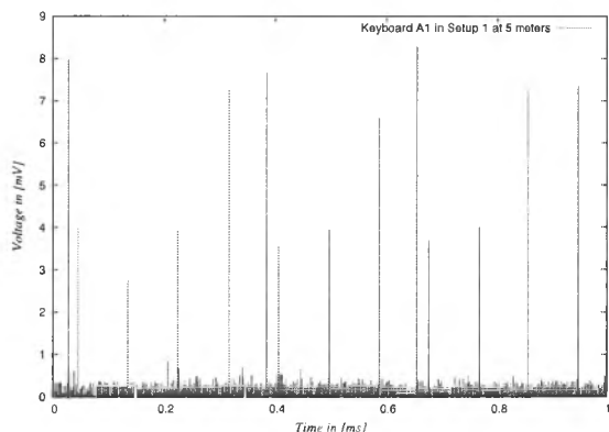
Figure 7: Band-pass (105-165MHz) filtered signal of Figure 6.
