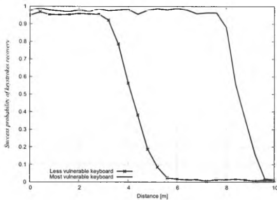
Figure 17: The success probability of the Generalized Transition Technique in the office, according to the distance between the keyboard and the antenna (biconical).
