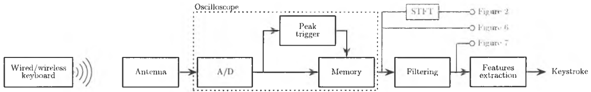
Figure 1: Diagram of our equipment for the experiments.
