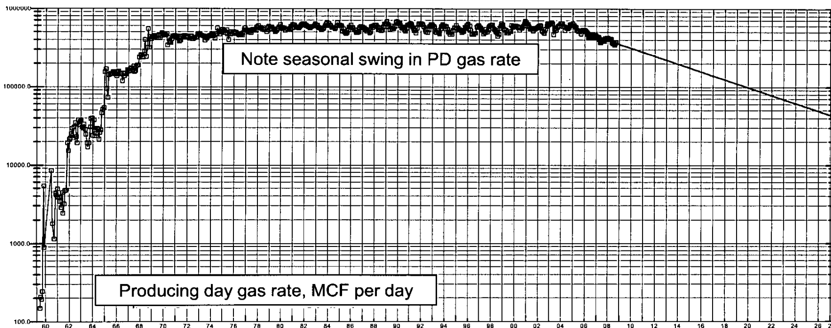
Figure 4. Decline curve projection based on data trend for production from all 28 Cook Inlet gas fields. Horizontal axis is time (1960-2028); vertical axis is producing day gas rate (MCF/day). Extrapolation line represents an annual average rate forecast, and does not illustrate seasonal fluctuation in demand.
