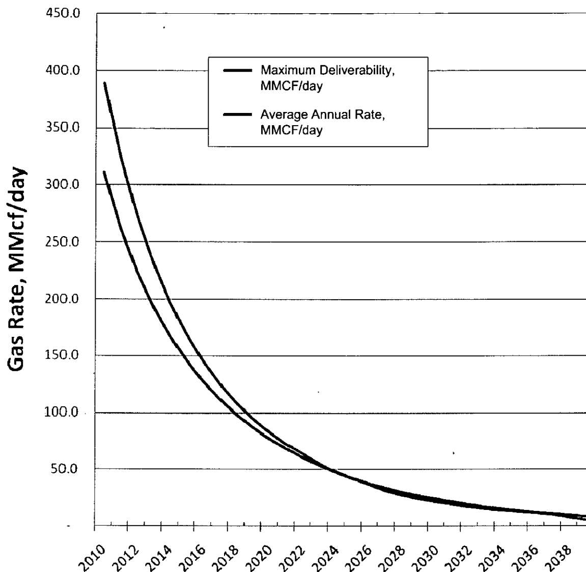
Figure 11. Peak maximum producing day deliverability compared to average annual rate from decline curve analysis.
