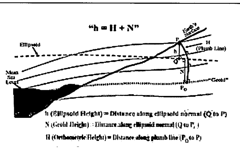
Figure 4. Geodetic formula for conversions between ellipsoid heights and orthometric heights.
