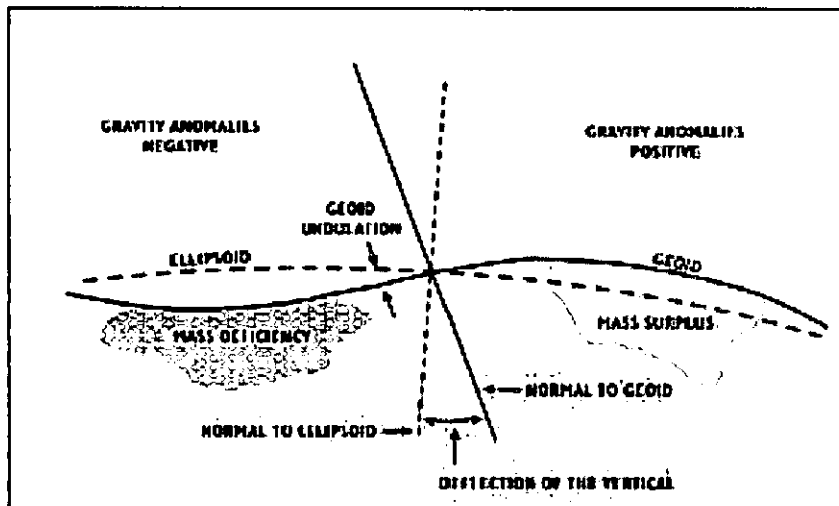
Figure 3. Ellipsoid, geoid, and geoid undulation (geoid height).
