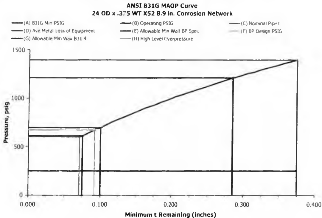
Figure E.10 MAOP versus Remaining Wall Thickness
