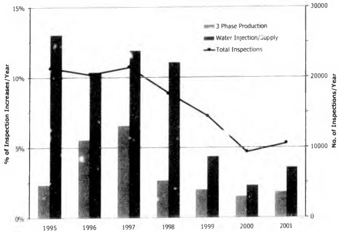
Figure E.7 Flow Line Internal Inspection Increase by Service
