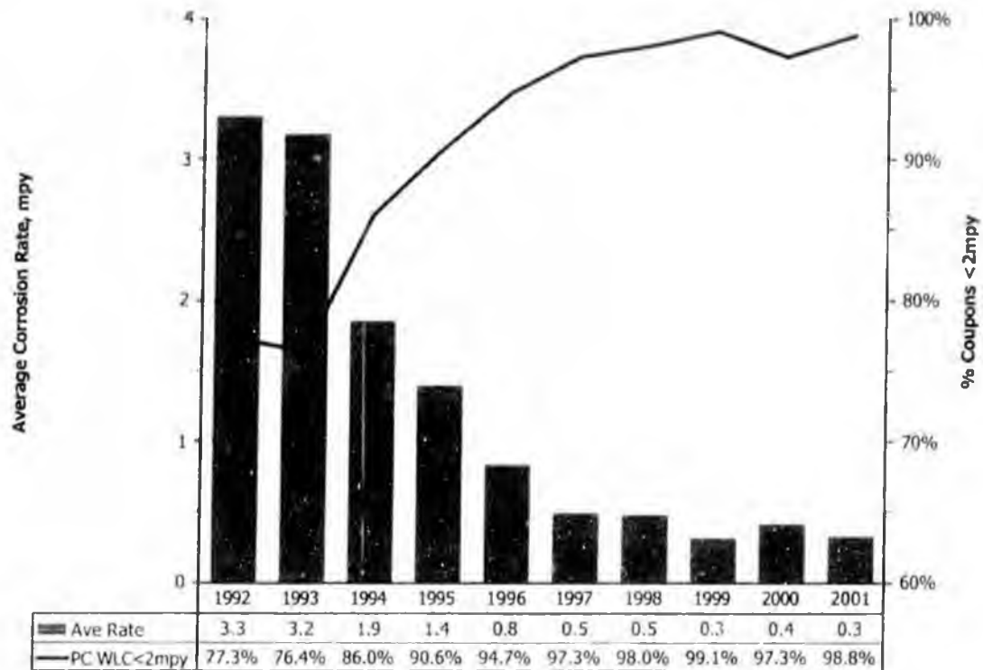
Figure C.1 Flow Line Corrosion Rate Trend 1992 to 2001
