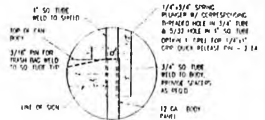
DETAIL 3 PIN & SUPPORT
