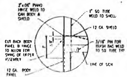
DETAIL 1 HINGE
