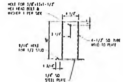
RECEPTACLE BASE-ELEVATION, PART 'B' SCALE 1 1/2"=1'-0"
