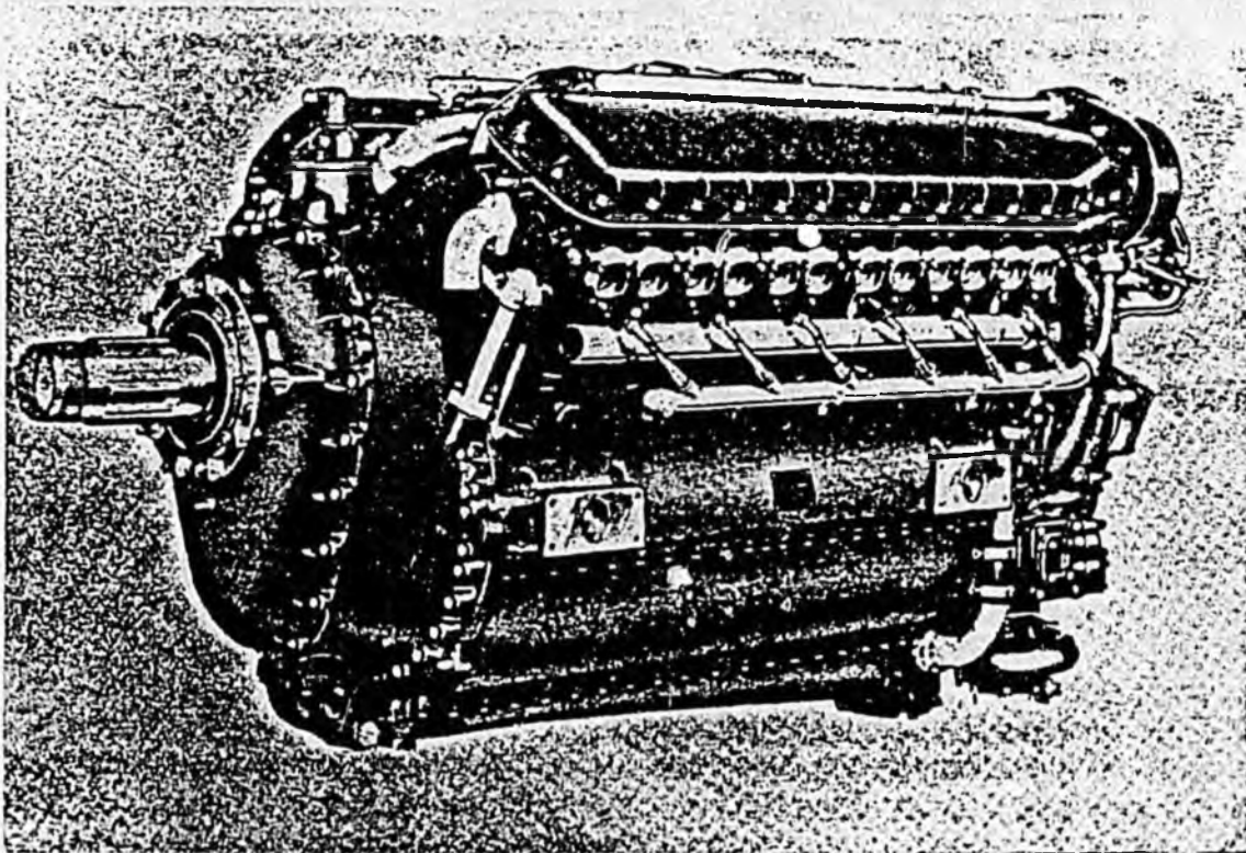
This is a P-38 Allison V-1710F series engine. Four dump areas were located in which these type of engines were buried in packing cylinders. ADGM
