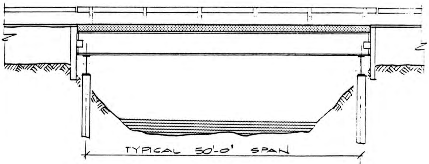
BRIDGE ELEVATION
