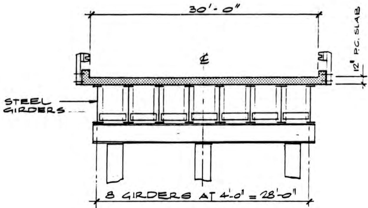
BRIDGE SECTION
