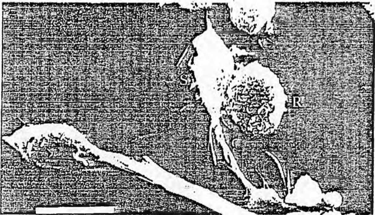
FIGURE 6. Scanning electron micrograph of untreated UICC chrysotile asbestos fibers associated with hovine alveolar macrophages: cells (S) were often observed spread along asbestos fibers with additional rounded macrophages (R) nearby (1940 \times , bar = 10 \mu m).
