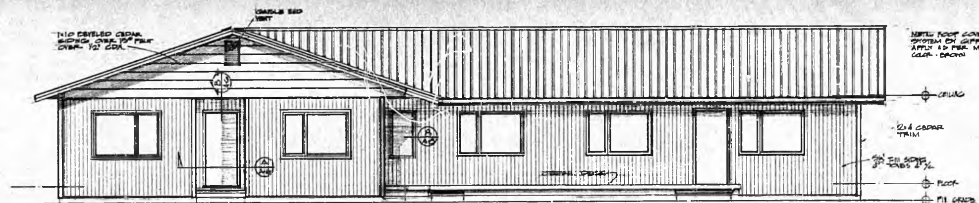
WEST ELEVATION 1/4" = 1'-0"
