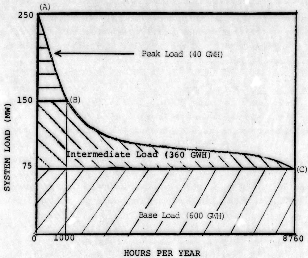
FIGURE 2 HYPOTHETICAL LOAD DURATION CURVE
