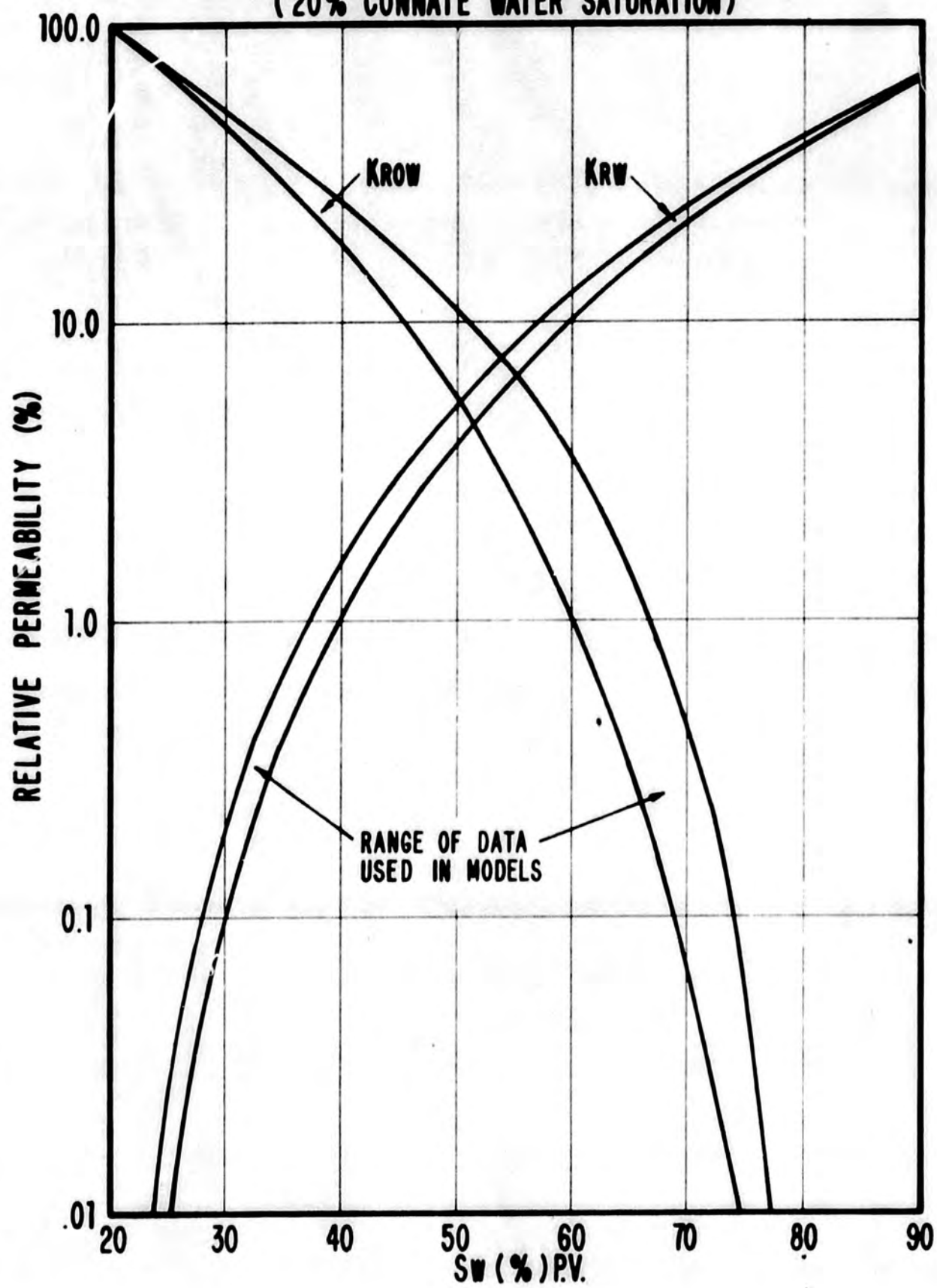
FIGURE 9 SADLEROCNIT WATER - OIL IMBIBITION RELATIVE PERMEABILITY (20% CONNATE WATER SATURATION)
