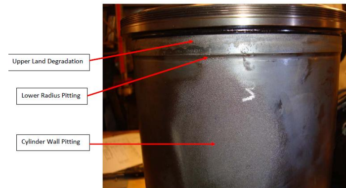
Figure 1: Fairweather Engine ME#3, 3 O'clock position, land, radius and wall degradation.
