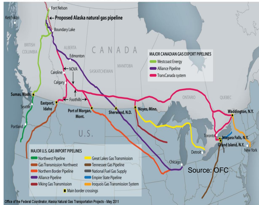
MAJOR CANADA, U.S. EXPORT-IMPORT GAS PIPELINES
