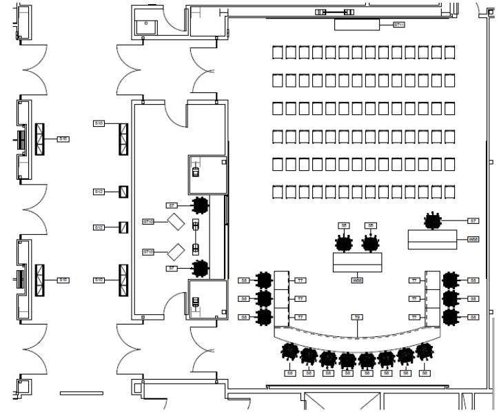
1 ENLARGED FURNITURE PLAN - AUDITORIUM LAYOUT 1 1/4" = 1'-0"
