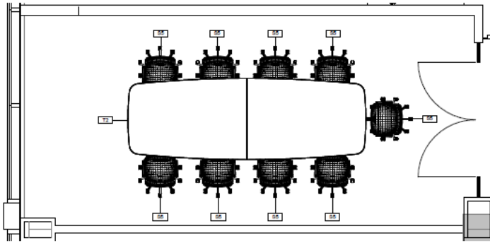
2 ENLARGED FURNITURE PLAN - TYPICAL CONFERENCE ROOM 1/2" = 1'-0"
