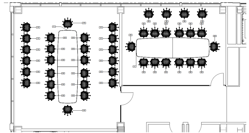
1 ENLARGED FURNITURE PLAN - CONFERENCE ROOMS LEVEL 2 1/8" = 1'-0"
