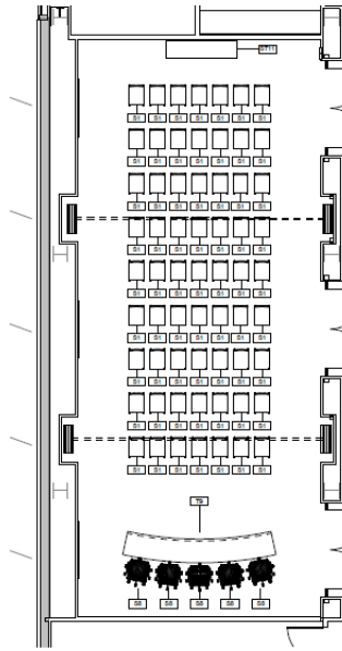
2 ENLARGED FURNITURE PLAN - LARGE MEETING SPACE 1/4" = 1'-0"
