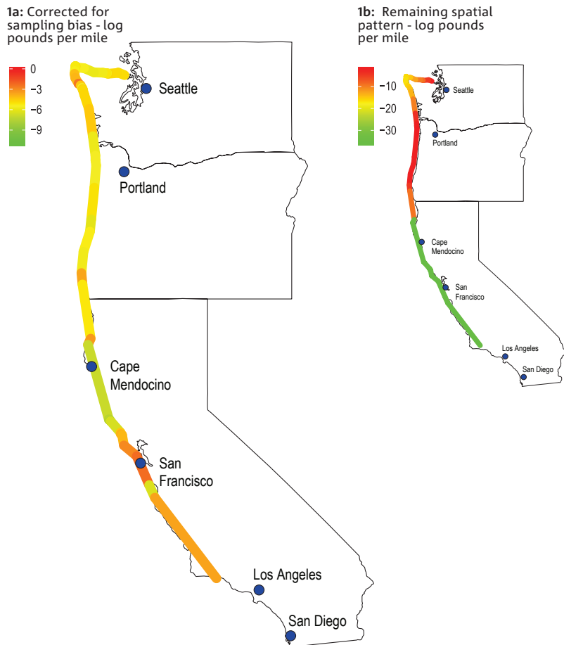
Figures 1a and 1b: Shoreline debris load based on NOAA MDP accumulation data. The ribbon on the left shows the relative amount of debris after accounting for sampling bias, while the ribbon on the right shows the remaining levels of debris after accounting for sampling bias, population density and other drivers, possibly indicating a greater offshore component to the debris north of Cape Mendocino.
